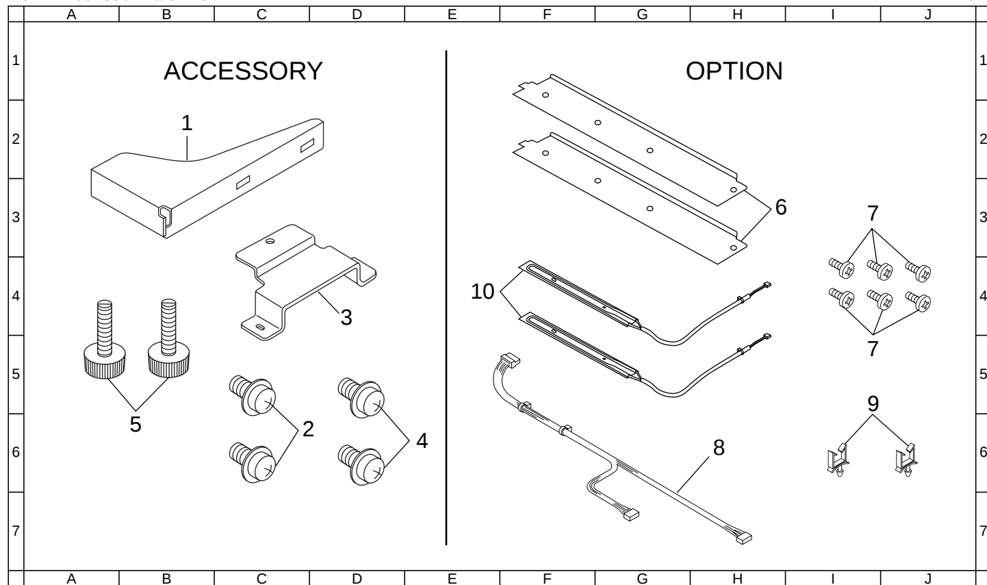
FIG. 4 ACCESSORY & OPTION
