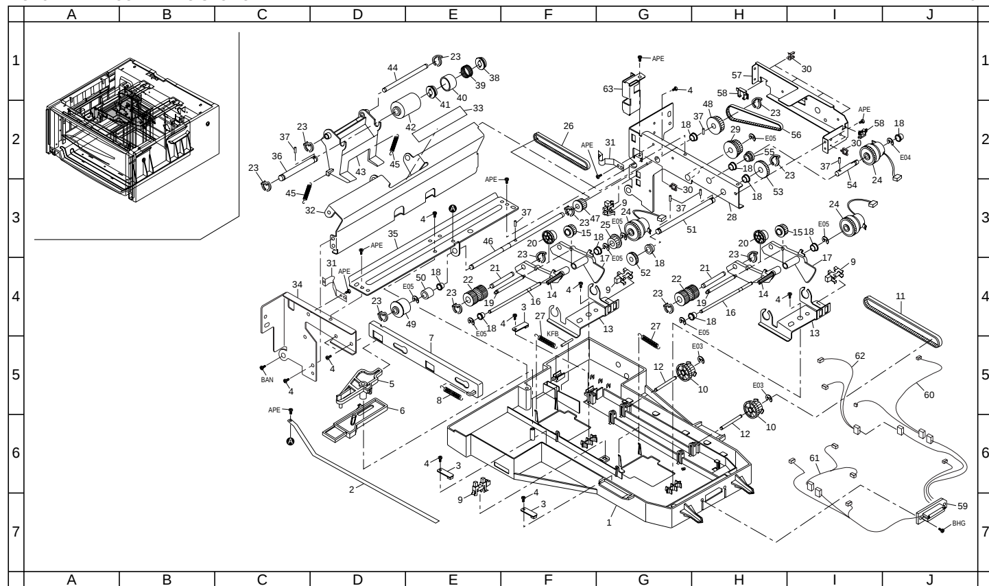
FIG. 3 PAPER CONVEYING SECTION
